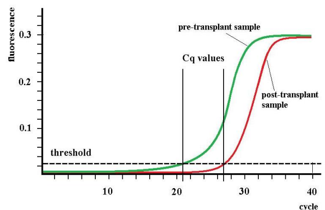
Figure 2. qPCR fluorescence signal curve
